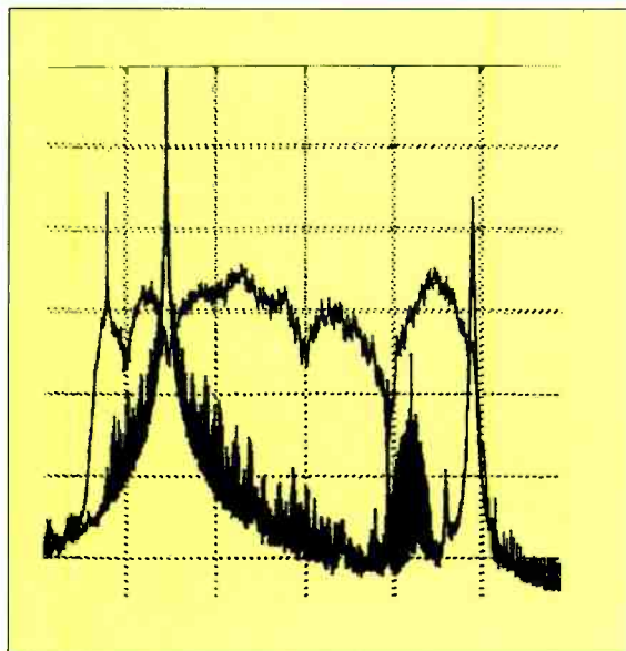
Figure 2. The NTSC and HDTV spectra as they might appear at the receiver.
