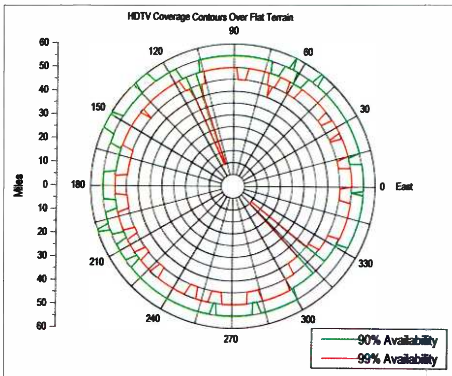
Figure 5. Antenna contours that would result when the installation of Figure 3 is combined with the power penalty of Figure 4.
