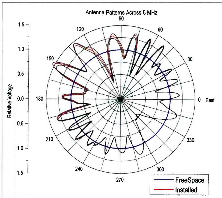
Figure 3. The radiation pattern of an omnidirectional antenna (Channel 38) after it is installed next to (8-foot separation) a tower with a 10-foot face.
