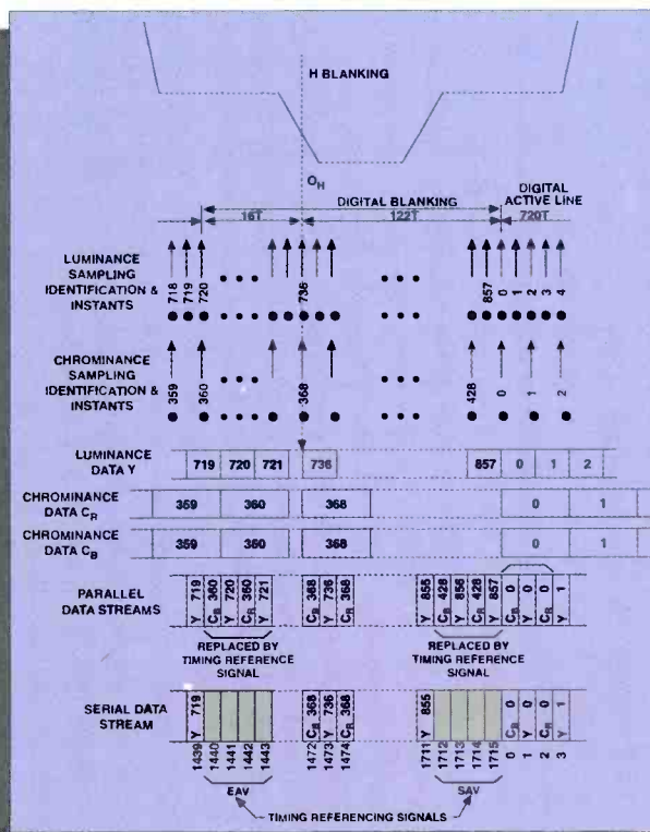
Figure 1. Structure of 4:2:2 digital sampling as per SMPTE 125M. (For more information, see "Transition to Digital," August 1995.)
