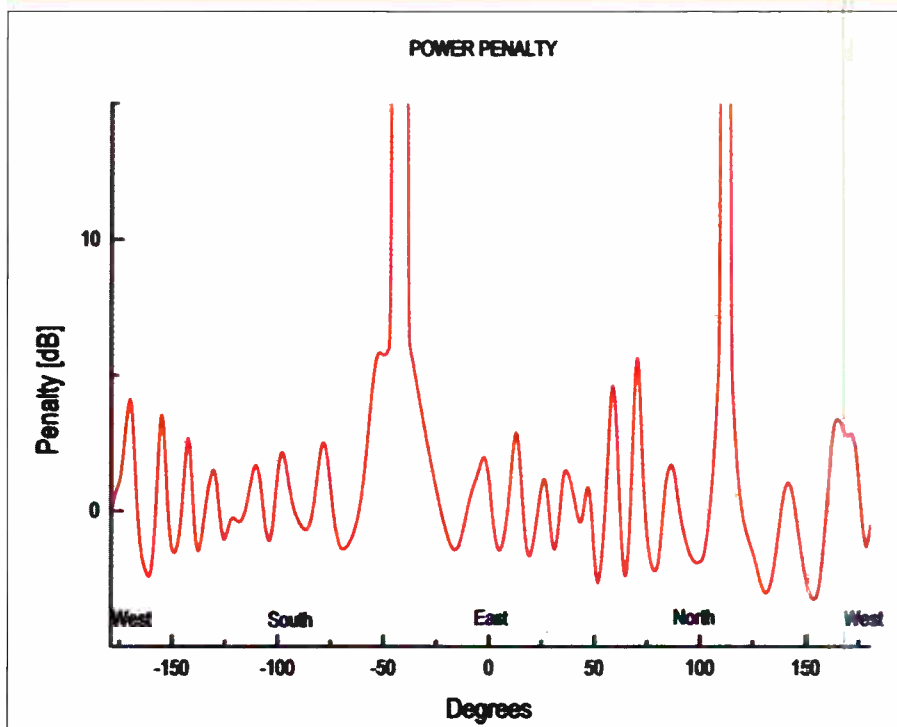
Figure 4. Power penalty that results from the pattern shown in Figure 3.
