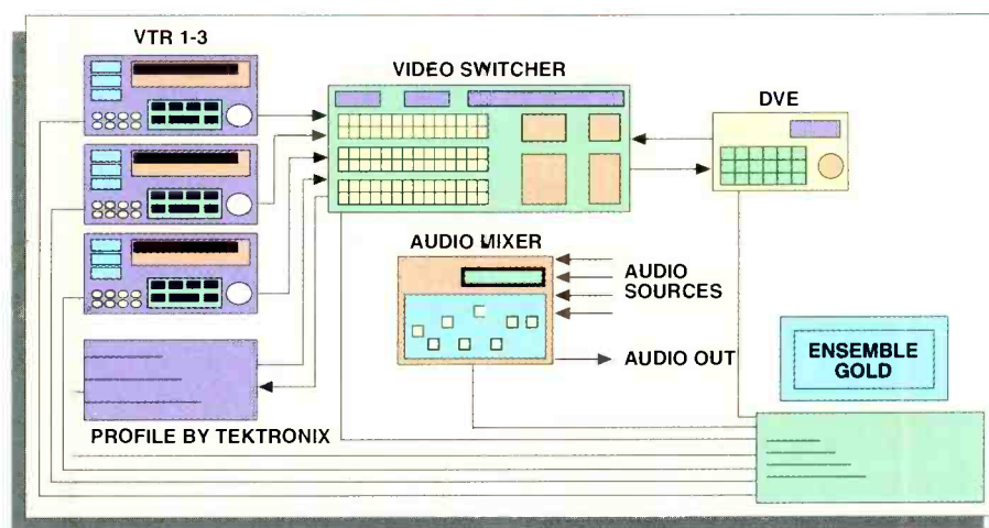
Figure 3. By incorporating the Ensemble Gold, this linear system has been expanded to include non-linear along with linear in one complete package. This system is using all external devices for DVE switching and audio, while the Tektronix Profile is providing digital betacam quality.
