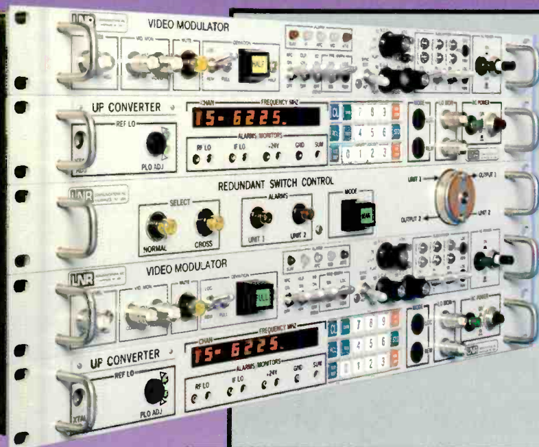
TYPICAL REDUNDANT CONFIGURATION
