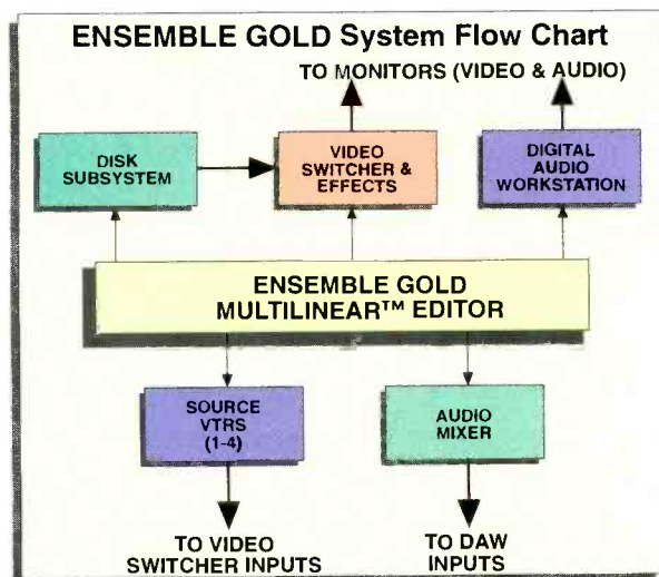
Figure 1. Basic system layout of a typical Ensemble Gold system.
