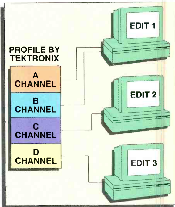
Figure 2. Depicted here is a non-linear editing network by Editing Technologies Corporation using Profile by Tektronix and the Ensemble Gold. It has two channels for AB on-line and two channels, one each, for two cuts-only suites. All three suites can work independently and access material as needed. Each system is configured to use specific channels as needed.
