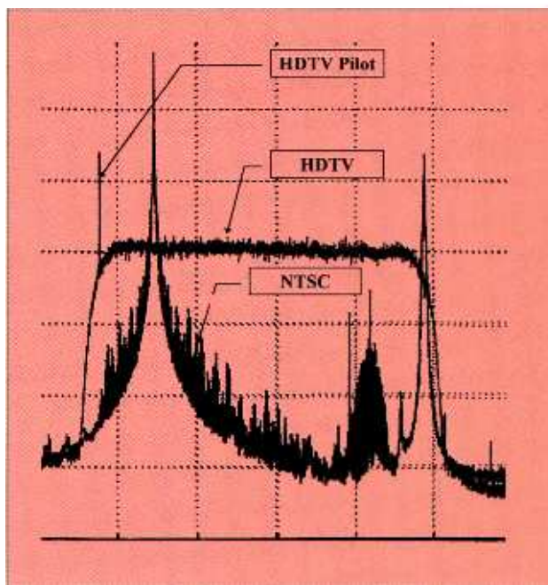
Figure 1. The spectra of undistorted NTSC and HDTV channels.
