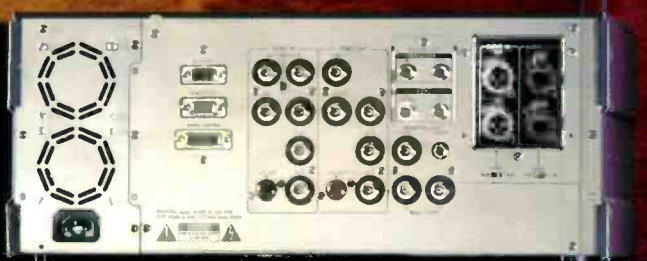
▼ Back panel BR-D85
