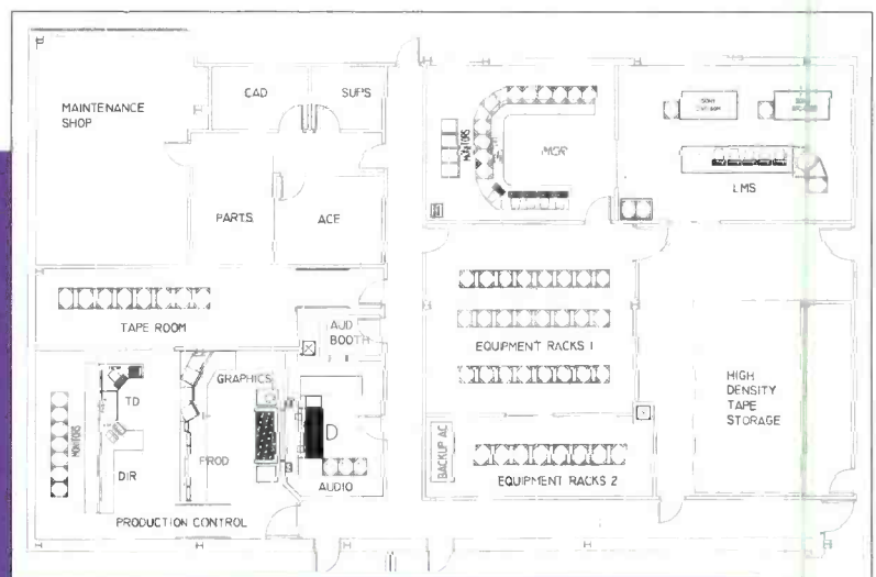
Figure 1. Simplified floor plan of the technical areas of the new KPTV building. All broadcast functions are built around a centralized technical core, which includes two equipment rooms and master control. (Courtesy of KPTV.)
